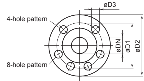
Flange dimensions in acc. with DIN EN 1092-2
