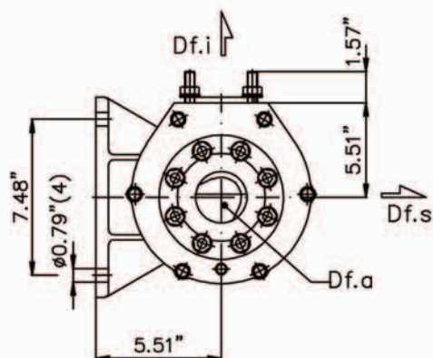
Suction view
