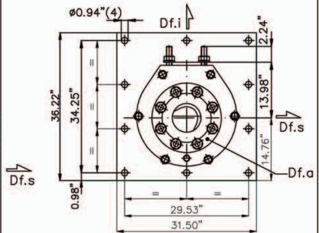
Suction view
