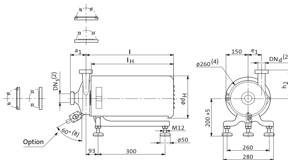
Annular housing with clamp ring (KLM)
