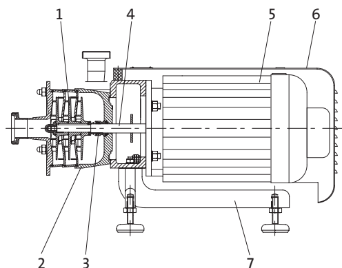
Fig. 5 Sectional drawing of Contra I Bloc-SUPER on combination foot
