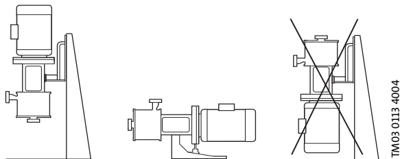
Fig. 31 Installation
