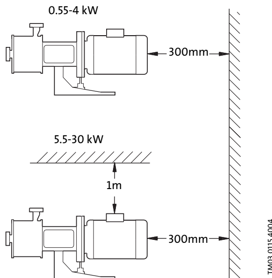
Fig. 33 Horizontal installation
