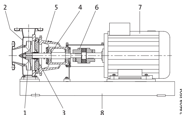
Fig. 10 Sectional drawing of MAXANA-CN on baseplate
