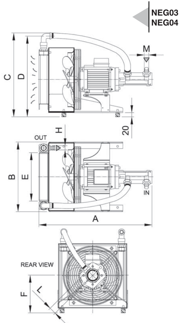
DIMENSIONAL CHART
